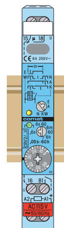
Connection diagram
