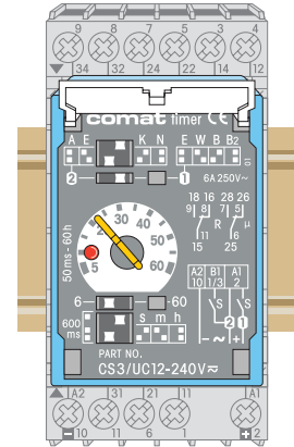
Connection diagram
