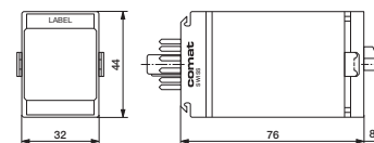
Dimensions [mm]
