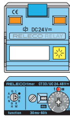
Time Delay Relay-Set Relay, Module and Socket
