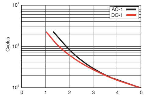
Fig. 2 Load limit curve
