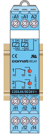
Connection diagram
